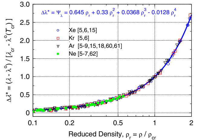
Fig. 5. Reduced, excess conductivity of the heavier noble gases versus reduced density.
