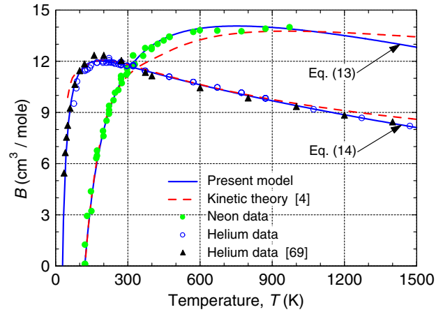
Fig. 15. Second virial coefficient of helium and neon versus temperature.
