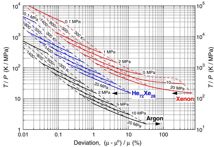
Fig. 34. Percent deviation between dynamic viscosity values calculated using the present pressure-dependence model and those calculated from the Chapman–Enskog kinetic theory of dilute gases.
