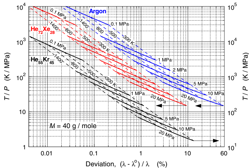
Fig. 32. Percent deviation between thermal conductivity values calculated using the present pressure-dependence model and those calculated from the Chapman–Enskog kinetic theory of dilute gases.
