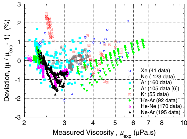
Fig. 7. Percent deviation between predicted and measured viscosities of dense noble gas mixtures at various temperatures and pressures.
