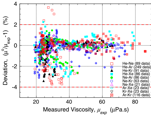
Fig. 20. Percent deviation between predicted and measured viscosities of binary mixtures of the noble gases at dilute density ( P \leq 0.1 MPa).
