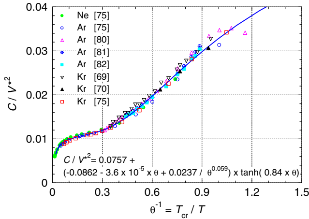
Fig. 14. Reduced third virial coefficients of the heavier noble gases versus reduced temperature.
