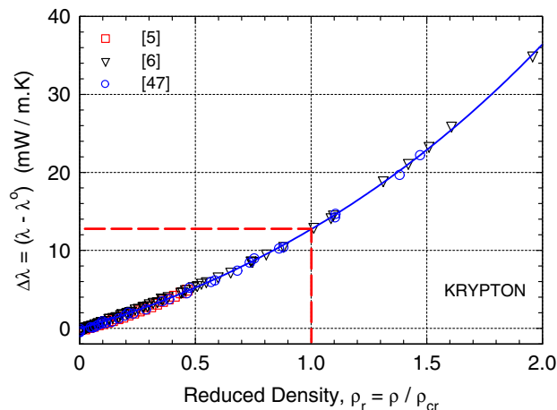
Fig. 4. Excess residual conductivity of krypton as a function of reduced density.
