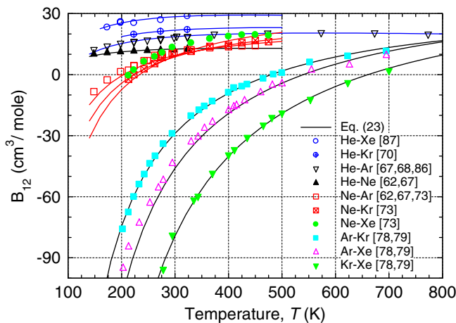
Fig. 18. Second virial interaction coefficients of noble gas mixtures.
