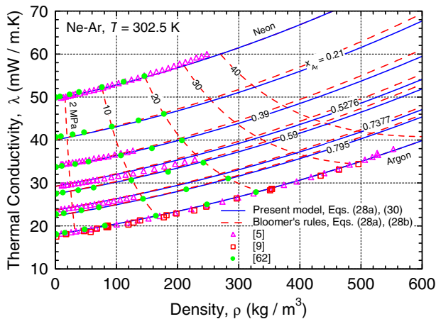
Fig. 27. Conductivity of neon–argon gas mixtures at 302.5 K and different pressures.
