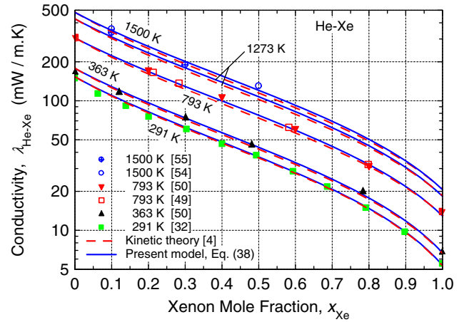
Fig. 24. Conductivity of helium–xenon binary mixtures at low-density ( P \leq 0.1 MPa).
