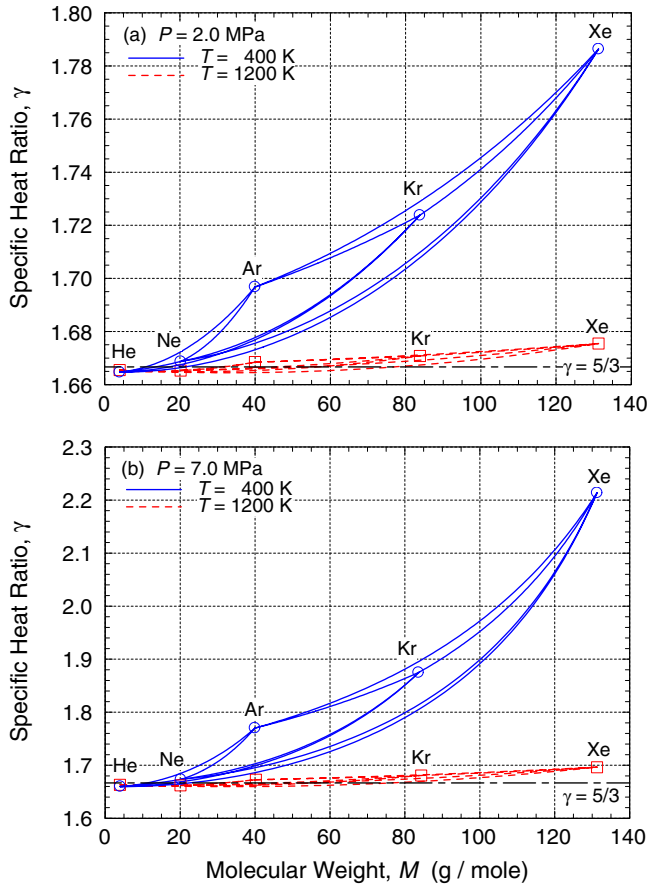
Fig. 30. Specific heat ratio of noble gases and their binary mixtures at pressures of 2 and 7 MPa.
