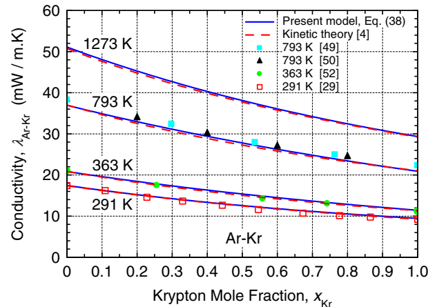
Fig. 25. Conductivity of argon–krypton binary mixtures at low-density ( P \leq 0.1 MPa).
