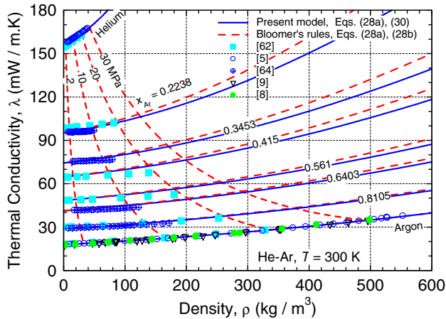
Fig. 26. Conductivity of helium–argon gas mixtures at 300 K and different pressures.
