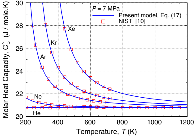
Fig. 16. Specific heat at constant pressure of the pure noble gases at 7.0 MPa.
