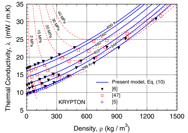
Fig. 12. Thermal conductivity of krypton as a function of pressure and temperature.
