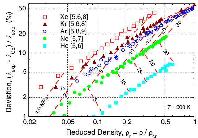
Fig. 1. Thermal conductivity of dense noble gases.
