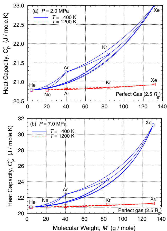
Fig. 29. Molar heat capacity of noble gases and their binary mixtures at pressures of 2 and 7 MPa.
