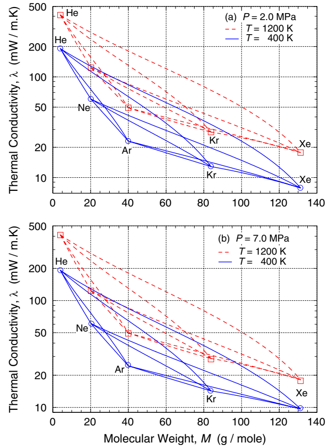
Fig. 31. Thermal conductivity of noble gases and their binary mixtures at pressures of 2 and 7 MPa.
