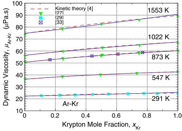
Fig. 22. Viscosity of argon–krypton binary mixtures at low-density ( P \leq 0.1 MPa).
