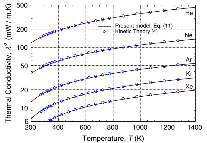
Fig. 9. Thermal conductivity of the pure noble gases at dilute density/atmospheric pressure.
