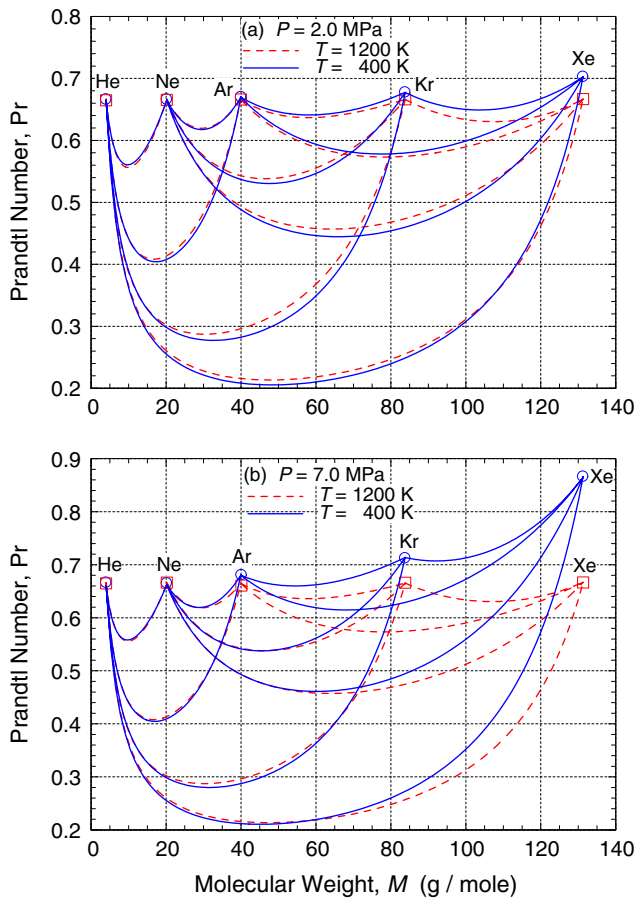
Fig. 35. Prandtl number of noble gases and their binary mixtures at pressures of 2 and 7 MPa.
