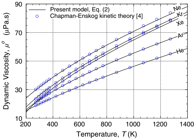
Fig. 6. Dynamic viscosity of the pure noble gases at dilute density/atmospheric pressure.
