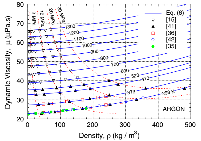
Fig. 8b. Viscosity of argon as a function of pressure and temperature at high temperature.
