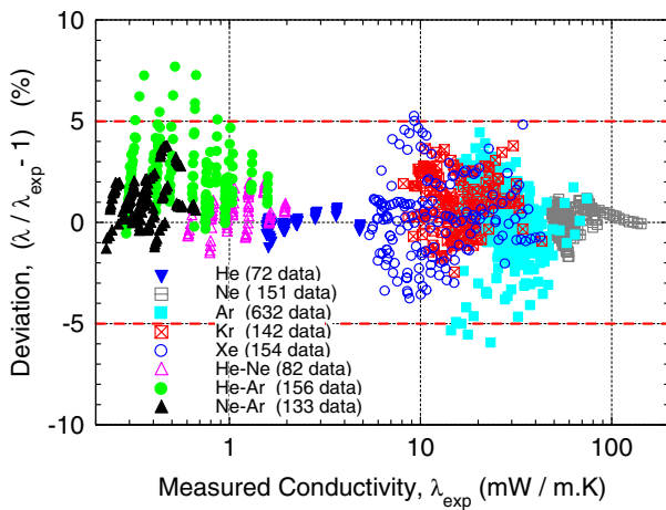
Fig. 10. Percent deviation between predicted and measured conductivities of dense noble gas mixtures at various temperatures and pressures.
