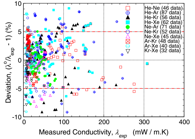
Fig. 23. Percent deviation between predicted and measured conductivities of binary mixtures of the noble gases at dilute density.
