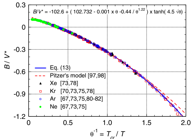
Fig. 13. Reduced second virial coefficients of the heavier noble gases versus reduced temperature.
