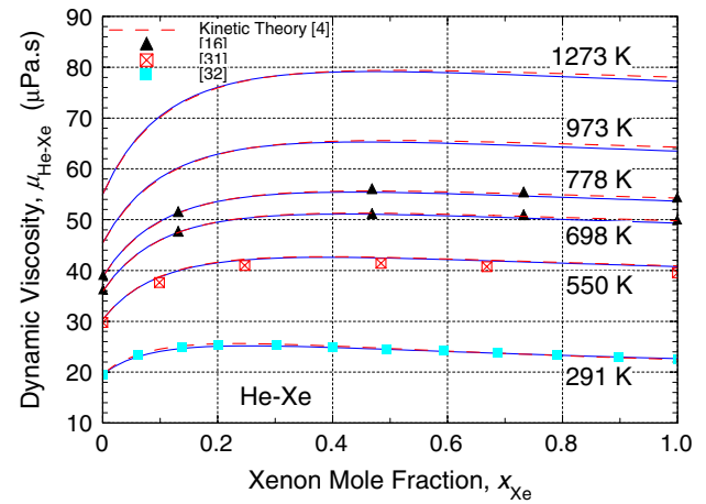
Fig. 21. Viscosity of helium–xenon binary mixtures at low-density ( P \leq 0.1 MPa).
