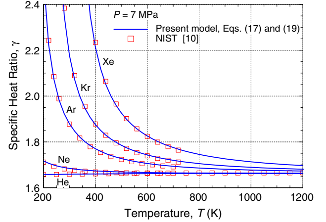
Fig. 17. Specific heat ratio of the pure noble gases at 7.0 MPa.
