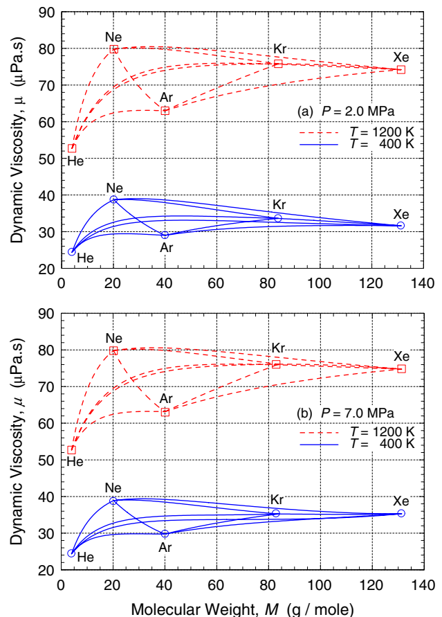
Fig. 33. Dynamic viscosity of noble gases and their binary mixtures at pressures of 2 and 7 MPa.
