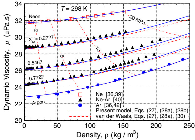
Fig. 19. Viscosity of Ne–Ar gas mixtures at 298 K and different pressures.
