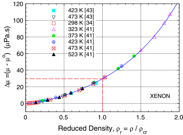
Fig. 2. Excess viscosity of xenon as a function of reduced density.
