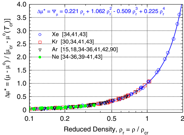
Fig. 3. Reduced, excess viscosity of the heavier noble gases versus reduced density.
