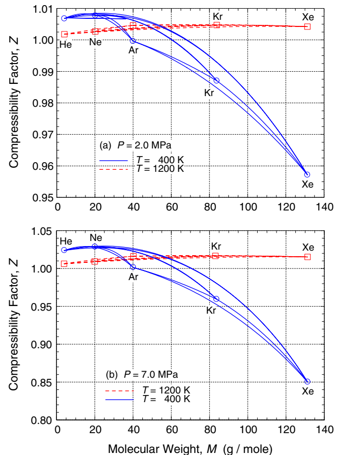
Fig. 28. Compressibility factor of noble gases and their binary mixtures at pressures of 2 and 7 MPa.
